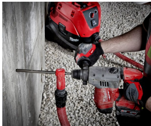
FIGURE 8— MILWAUKEE VACUUM BIT SYSTEM
